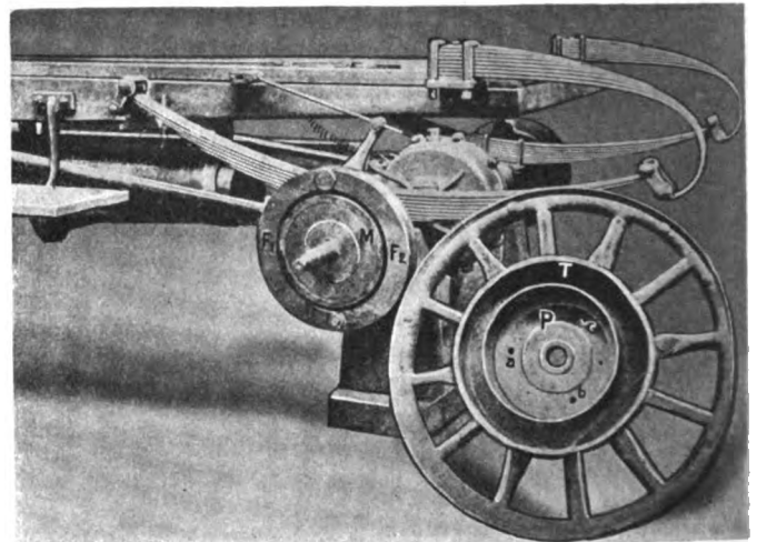
View of Rear Construction, with Wheel Removed.
